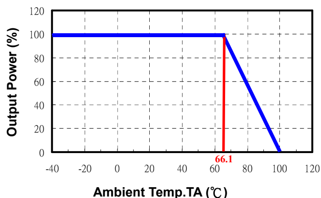
BWC40W Series Power Derating Curve with Heatsink (5)
